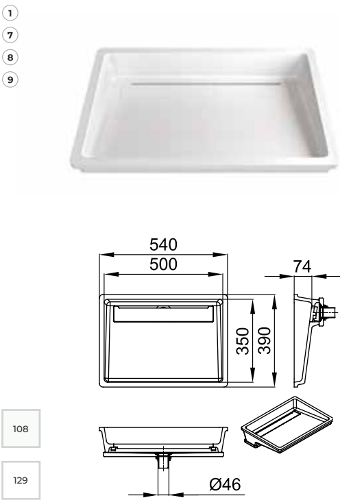
NEW KIARA 500 V-UN 500 mm / 350 mm / 74 mm / ø46 mm
